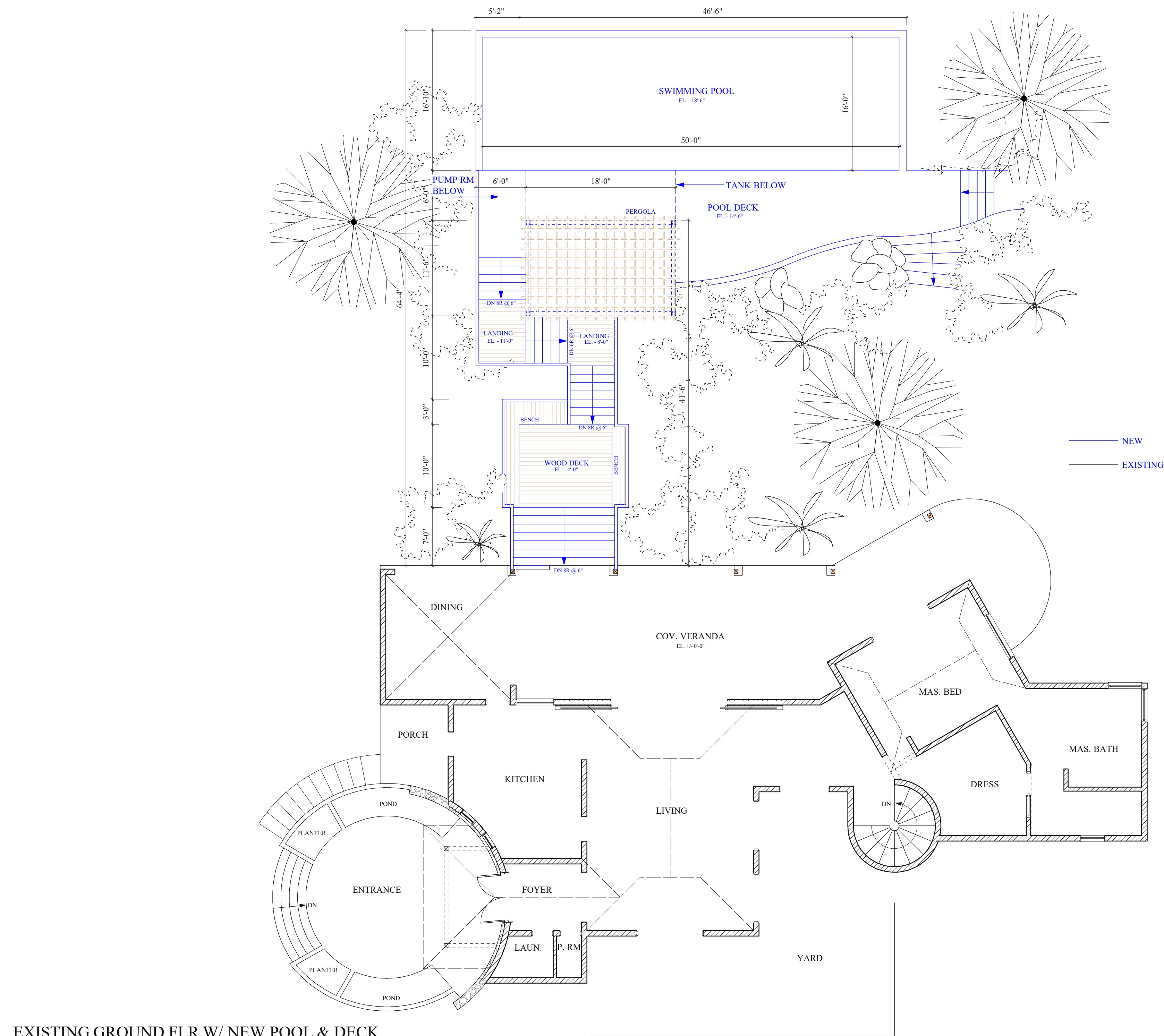
EXISTING GROUND FLR W/ NEW POOL & DECK
